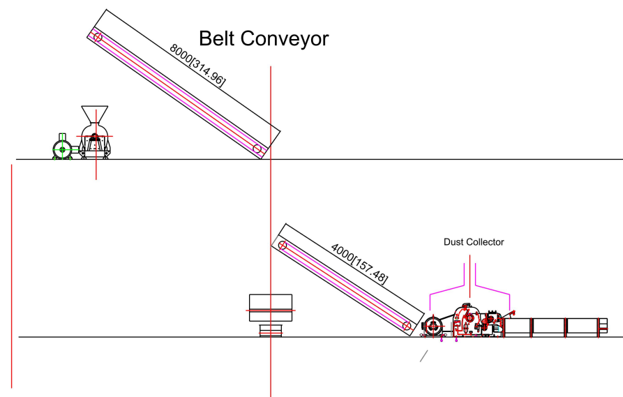
Vertical Layout for pellet production line
